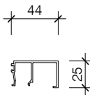
HAS020 AS104 GLAZING BEAD
