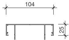
HAS010 AS104 HEAD/SILL TRACK
