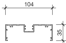
HAS015-35FLM AS104 MEDIUM POCKET CAPPING/FRAME
