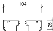
HAS014A AS104 GLAZING ADAPTOR
