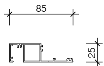
HAS019BA AS104 GLAZING BAR/SILL
