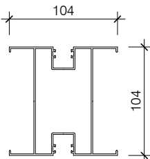
HAS024CP AS104 GLAZING CORNER POST
