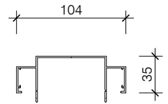
HAS010-SH AS104 SHADOWLINE HEADTRACK
