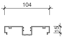
HAS012-MAP AS104 MULLION ADAPTOR
