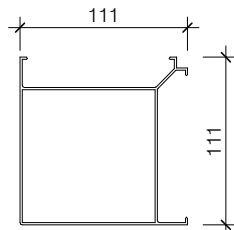
HAS024FCP AS104 FLUSH CORNER POST
