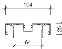
HAS014FM AS104 PLASTERBOARD POCKET CAPPING FRAME
