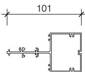
HAS021-B AS104 GLAZING SILL/TRANSOM
