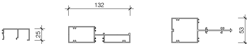
HAS320 AS132 GLAZING BEAD
