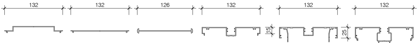
HAS311-SH AS132 SHADOW CAP
