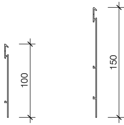
HAS009 100MM SKIRTING
