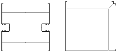
HAS324-CP AS132 GLAZED CORNER POST
