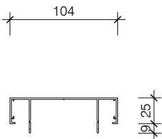
HAS010 AS104 HEAD/SILL TRACK
