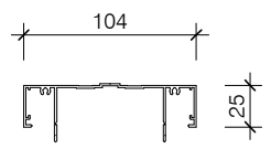
HAS010-R AS104 HEAD-SILL TRACK
