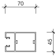
HAS004-GP70 CS45 GLAZING 70MM FRAME
