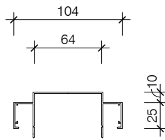
HAS010-SH AS104 SHADOWLINE HEADTRACK
