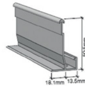
BULKHEAD TRIM DIAGRAM
