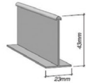
FLUSH FACE
