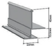
SCREWFIX MAIN RUNNER EDGE DIAGRAM
